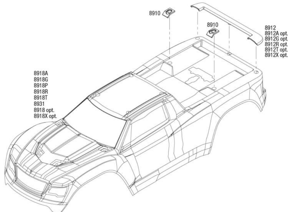
Completed Assembly (view from bottom)
